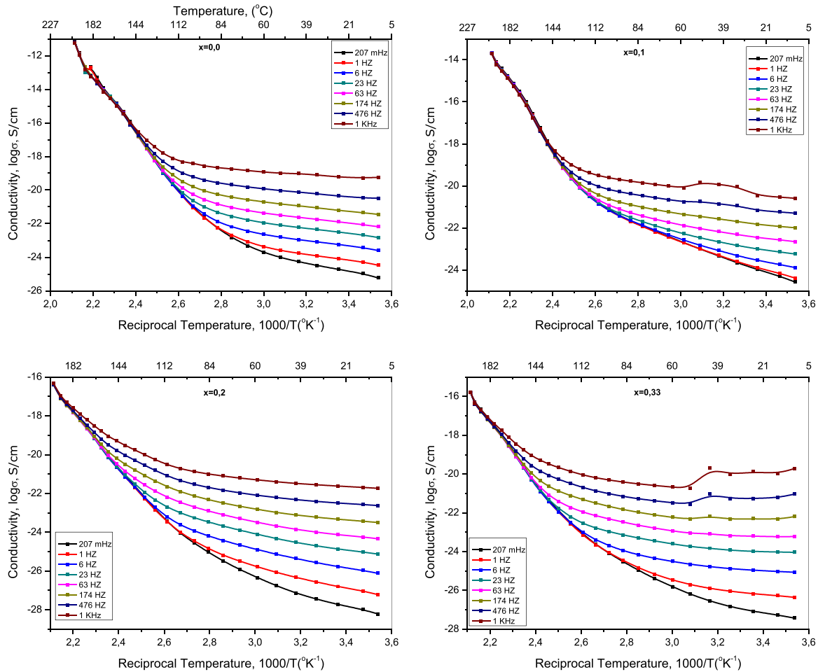
Fig. 4. Conductivity of Bi-La-Y substituted SrM ( 0.0 \leq x \leq 0.33 ) versus reciprocal temperatures for lower frequencies up to 1 kHz.
