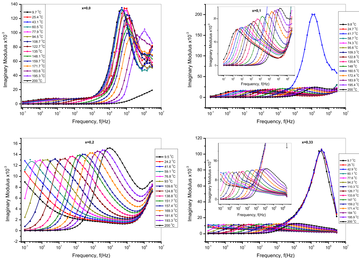
Fig. 15. Imaginary Modulus of Bi-La-Y substituted SrM ( 0.0 \leq x \leq 0.33 ) versus frequencies of up to 3 MHz for temperatures ranging from 10 °C to 200 °C.
