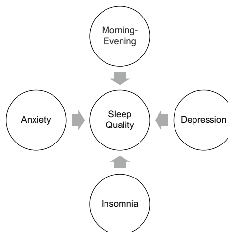
Figure 1: Research model
