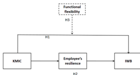
Fig. 1. Theoretical framework.
