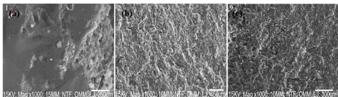
Fig. 12. SEM micrographs at 1000\times magnification for: (a) CT mortar; (b) CT-MF-10 mortar; and (c) CT-MF-30 mortar.
