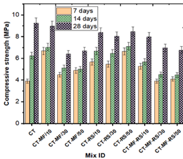
Fig. 10. Compressive strength of mortars.
