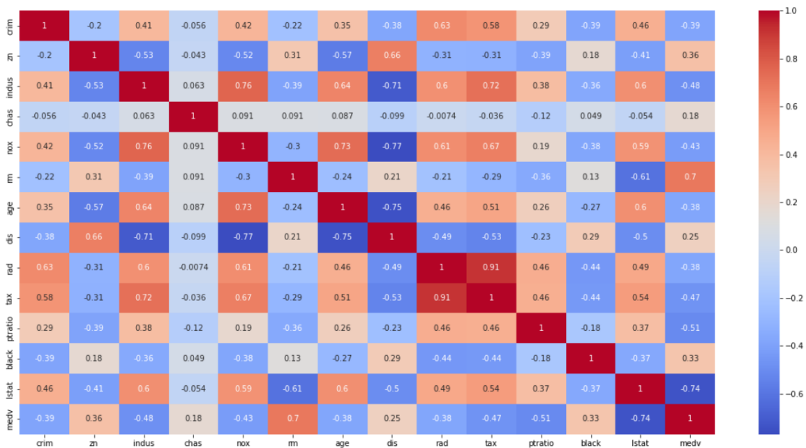
Fig. 5. Correlation matrix for all available features
