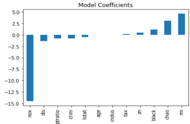
Fig. 3. Feature importance for all features
