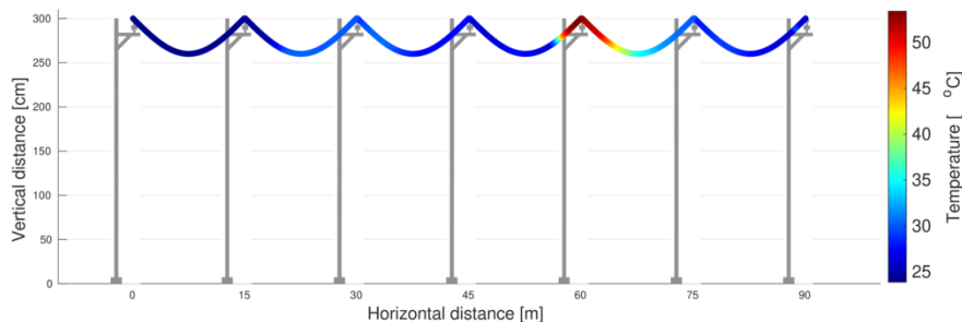
Fig. 5. Transmission line heatmap.
