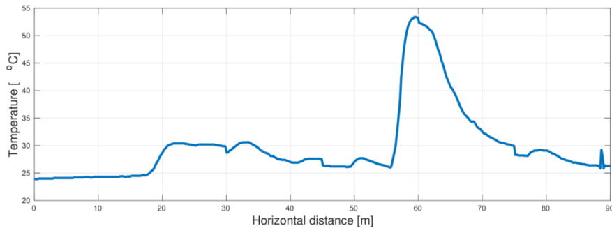
Fig. 4. Transmission line temperature.
